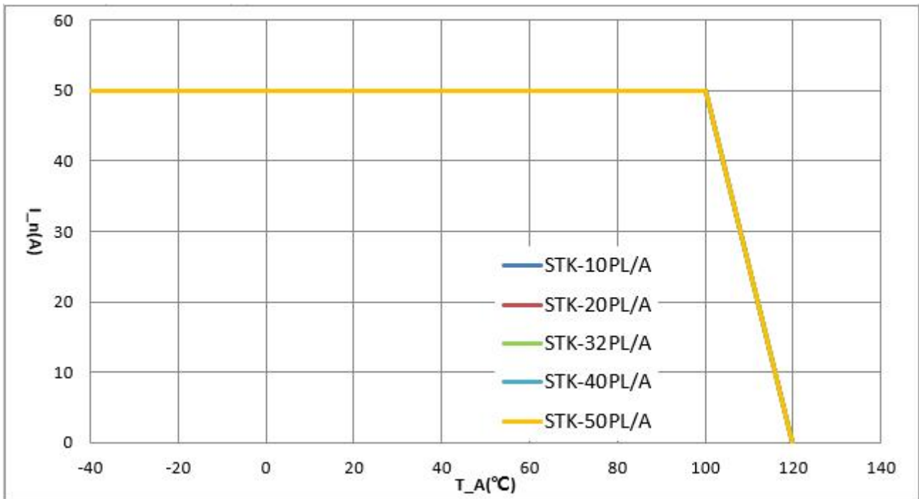
The dependence of maximum continues current of STK-PL/A current on the working temperature.
