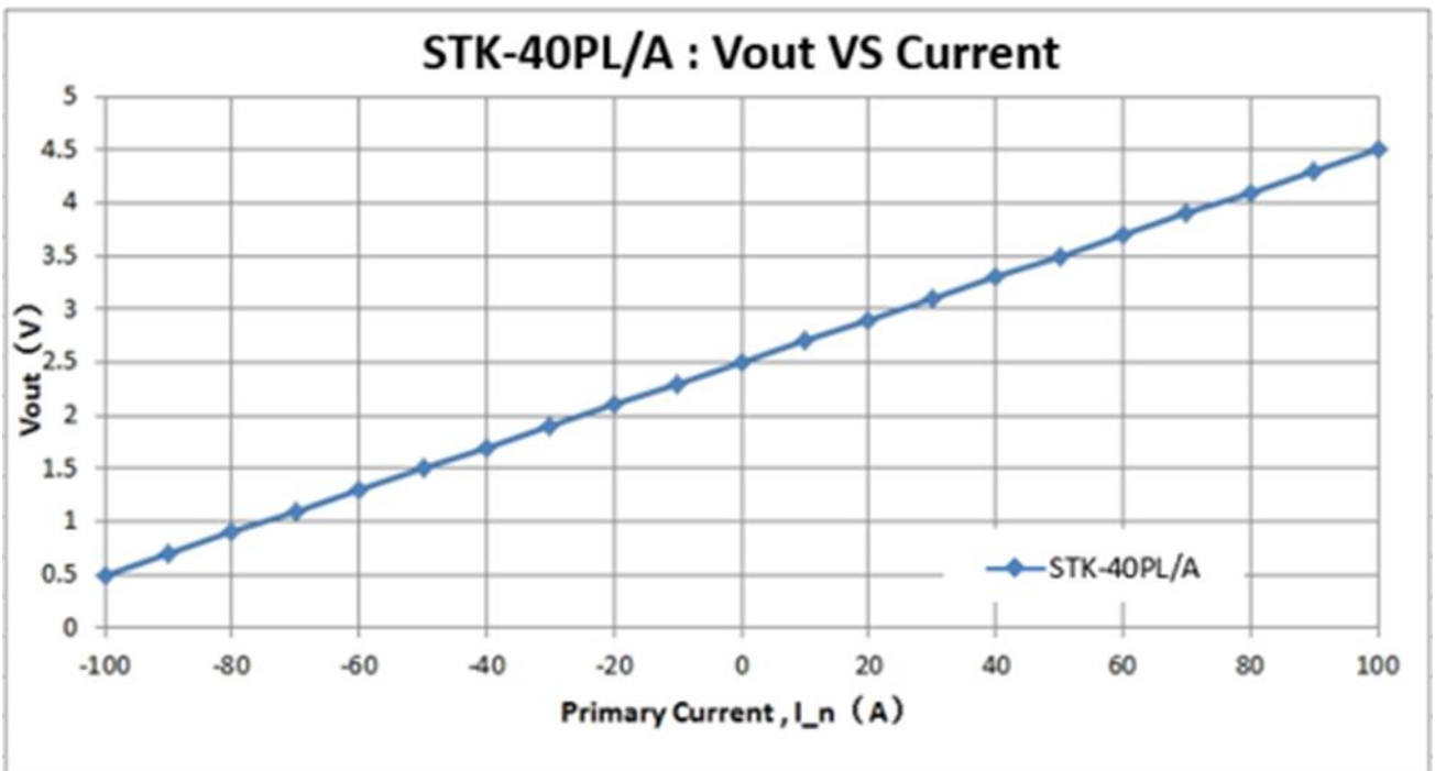
The dependence of Vout of STK-40PL/A on the primary current.
