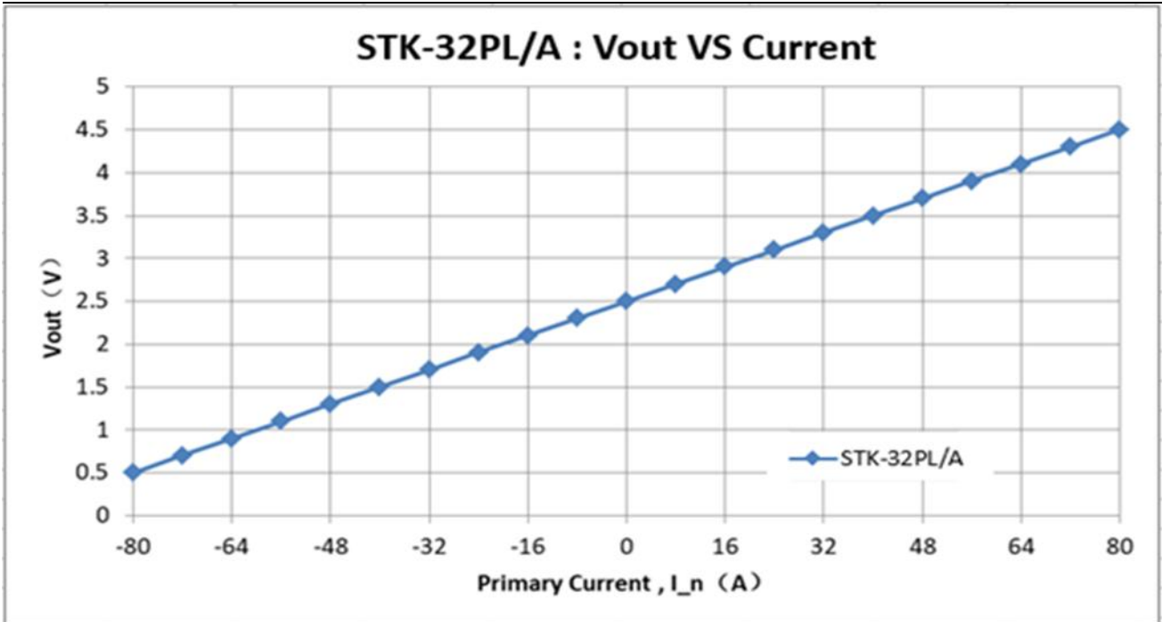
The dependence of Vout of STK-32PL/A on the primary current.
