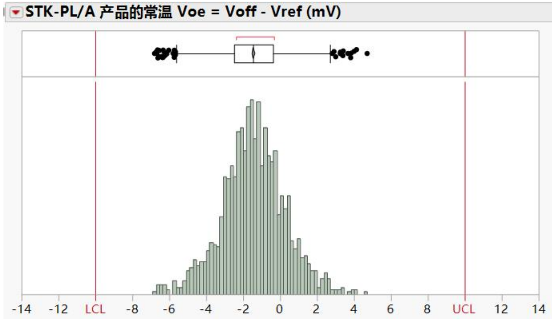
The distribution V_{oe} of STK-PL/A current sensor at 25°C.
