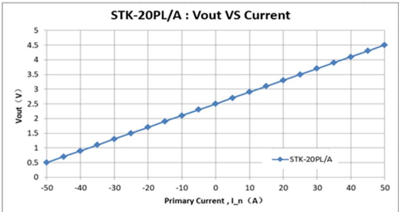
The dependence of Vout of STK-20PL/A on the primary current.
