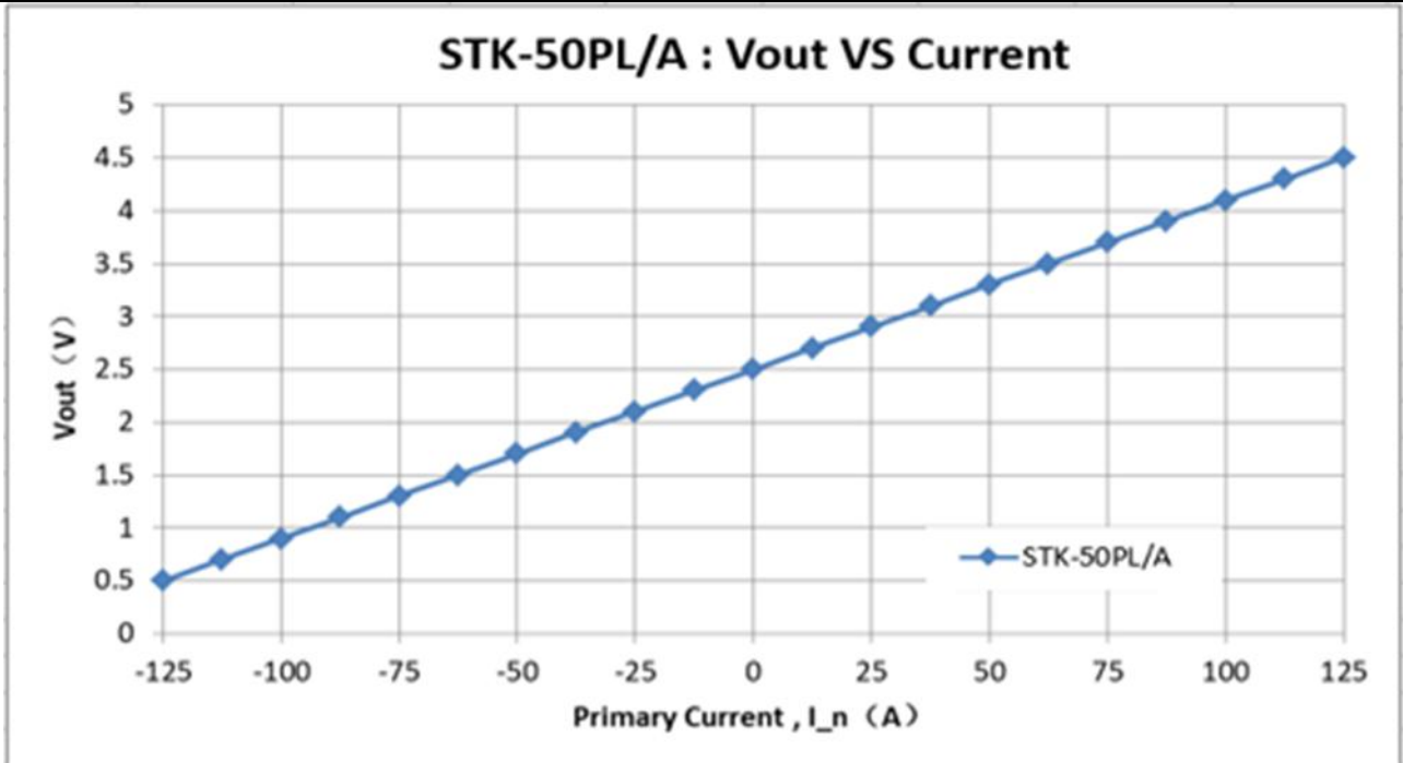
The dependence of Vout of STK-50PL/A on the primary current.
