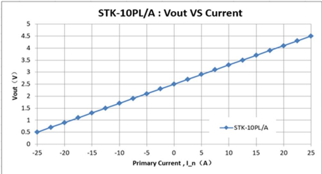
The dependence of Vout of STK-10PL/A on the primary current.
