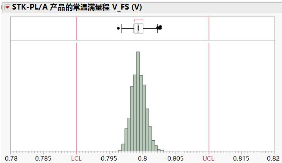
The distribution of V_{FS} OF STK-PL/A current sensor at 25°C.
