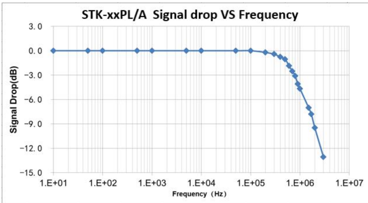
The frequency bandwidth of STK-PL/A series current sensor. The bandwidth of current sensor is DC ~ 400 kHz (-3dB).
