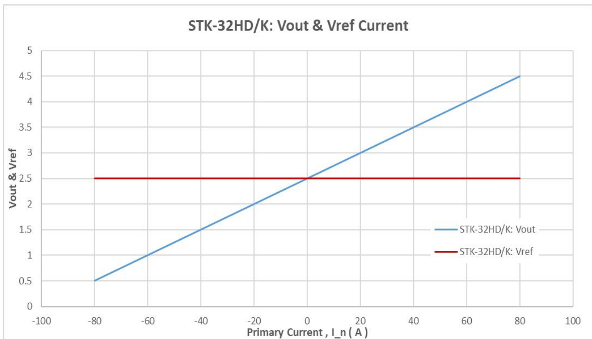
The dependence of Vout&Vref of STK-32HD/K on the primary current.
