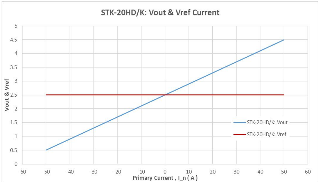
The dependence of Vout&Vref of STK-20HD/K on the primary current.
